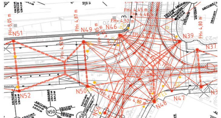
Traction line plan for a streetcar crossing
